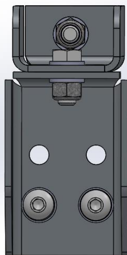
Fig 6: Tacoma Bracket kit Assembly Front View
